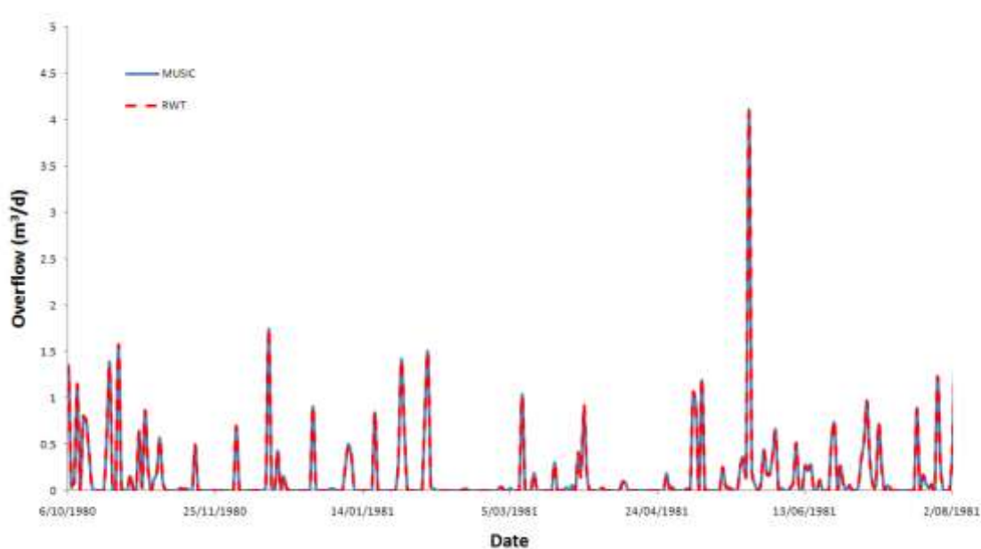
Figure 3. Comparison of overflow rate MUSIC and the modified RWT models.
