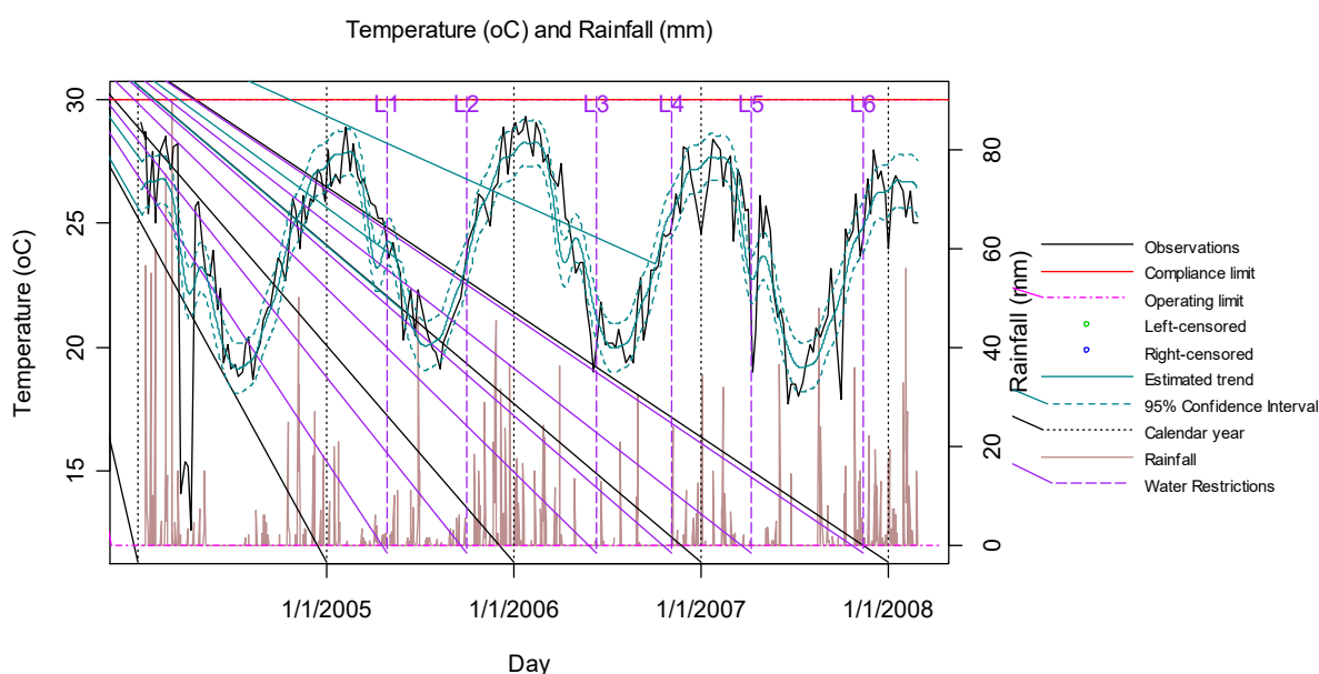
Figure 11 Plot of Effluent Temperature Recorded at Bundamba WWTP
