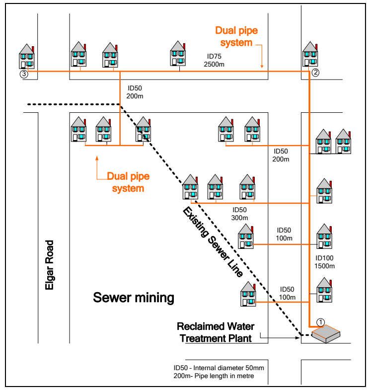
Figure 3: Cluster scale reclaimed water reuse system (Source: Sharma et al, 2005)
