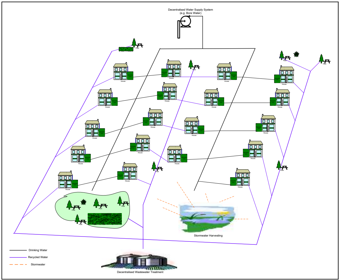
Figure 4: Development scale decentralised systems
